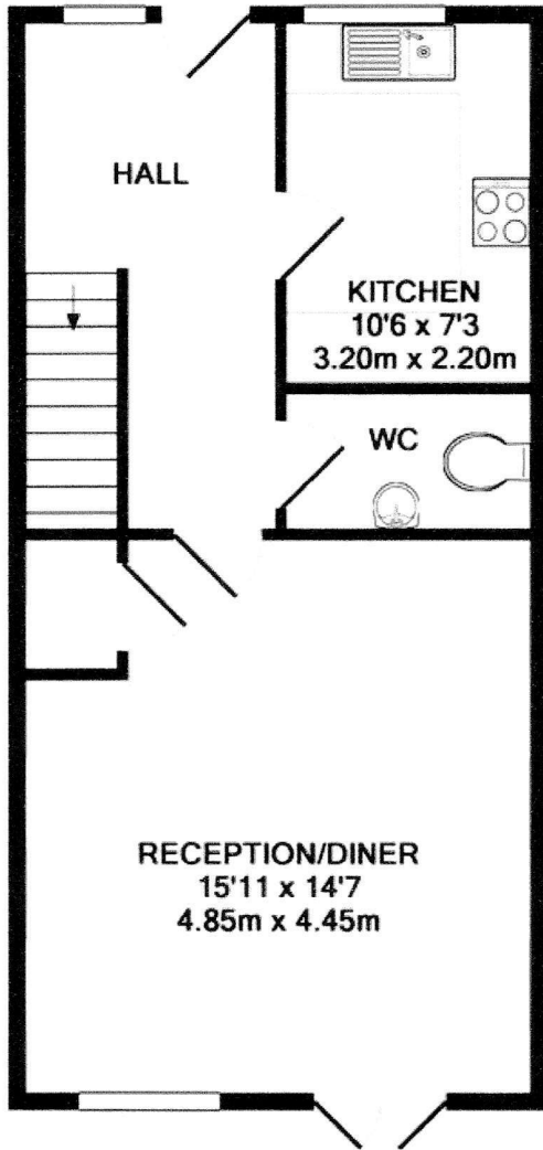
GROUND FLOOR APPROX. FLOOR AREA 445 SQ.FT. (41.4 SQ.M.)
